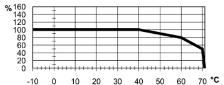
Output derating Curve Continuous Load
